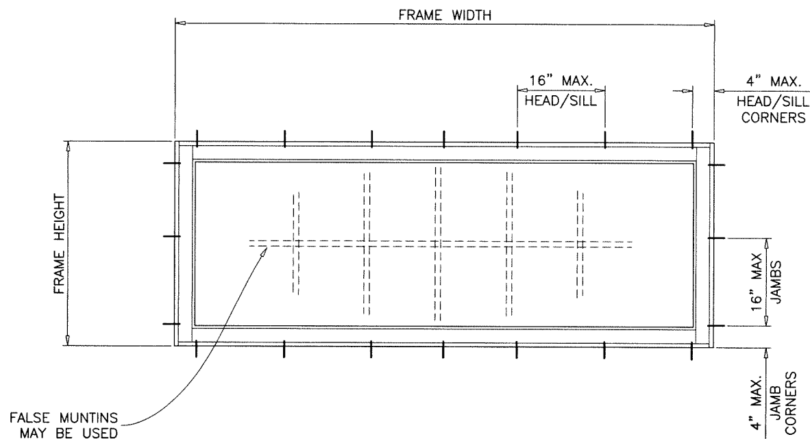
TYPICAL ELEVATION
