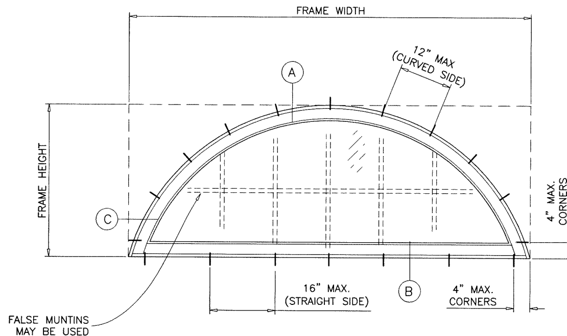
TYPICAL ELEVATION
