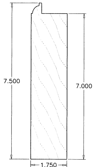
⑦ TOP RAIL
