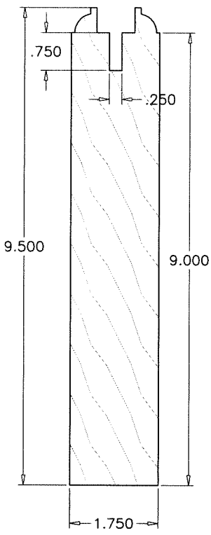
⑧ BOTTOM RAIL
