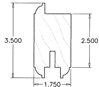
⑤ MID - RAIL
